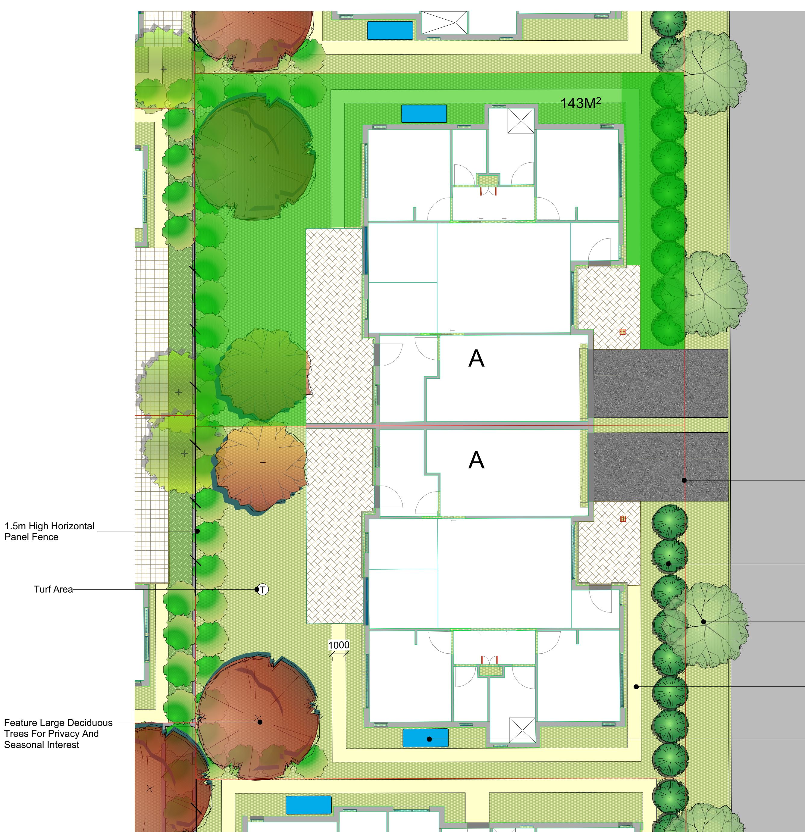
1. UNIT A TYPICAL FLOOR PLAN 1: 100 @ A1
